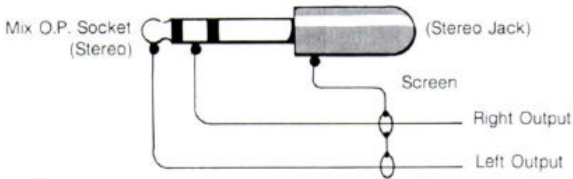
Hi-Fi Connection
