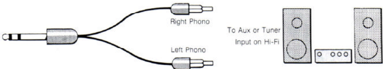
Stereo P.A. Connection
