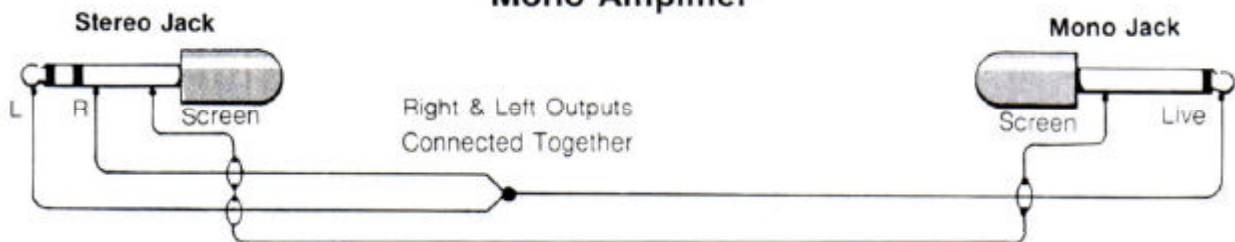
Mono Amplifier
